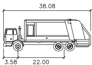
Rear-Load Garbage Truck
