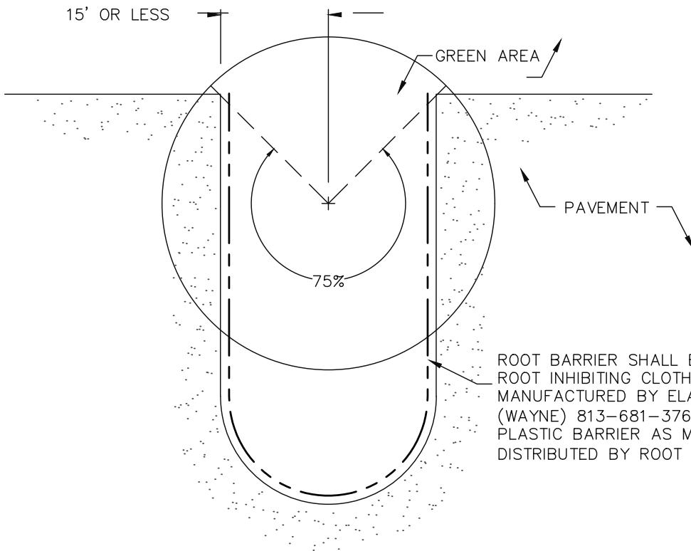
PLAN VIEW
