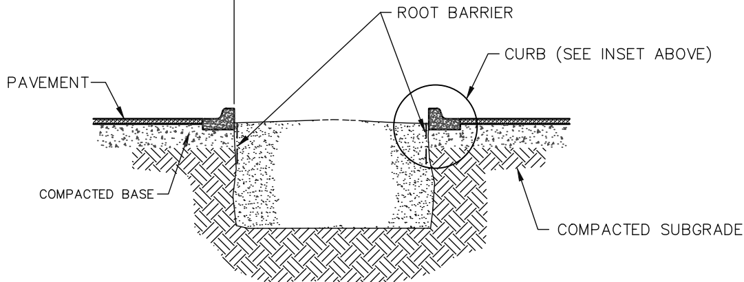
SECTION VIEW
